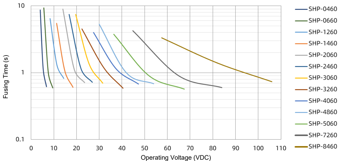
SHP 60 A Controlled Fusing Time Curve
