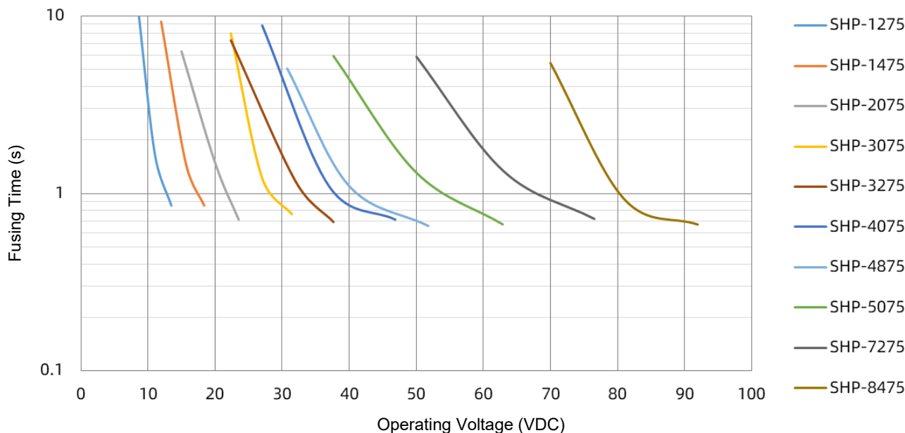
SHP 75 A Controlled Fusing Time Curve
