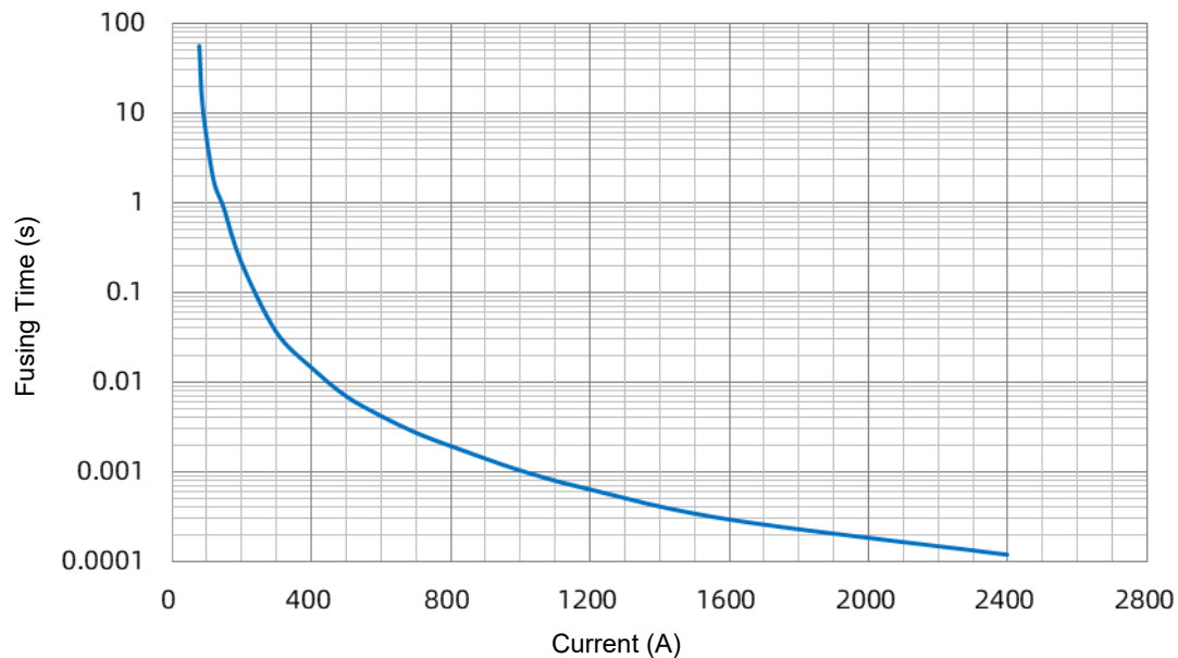
SHP 45 A Current-Time Curve
